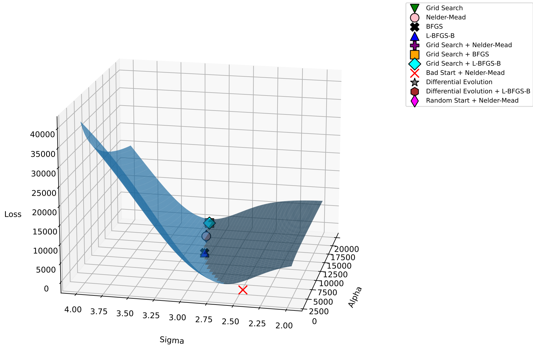
Loss Surface
